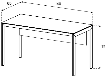
WD1 (Work Desk 1)
