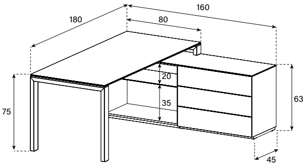
LD1 (L Desk 1)
