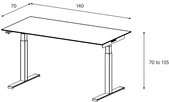
WLM (Work Lift Medium)
