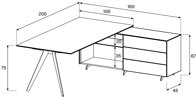
DP1 (Desk Plus 1)
