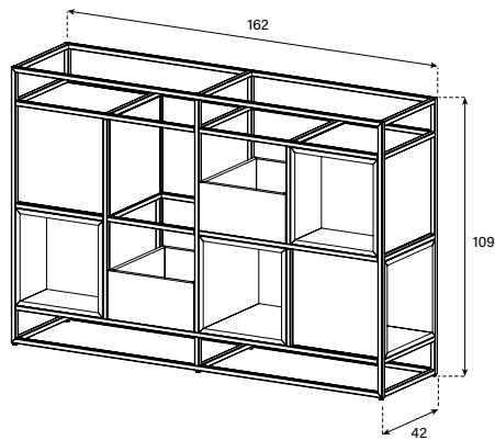
DVC (Divider Cabinet)
